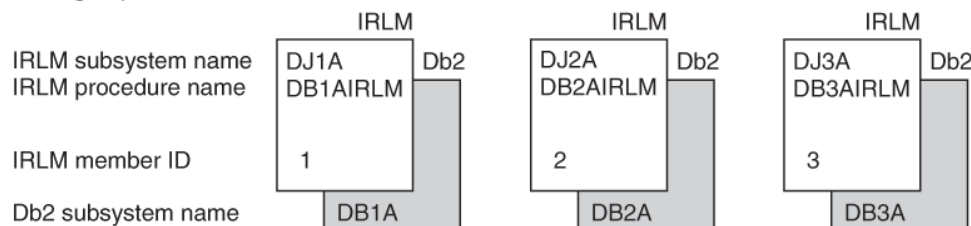
Figure 80. Relationship between Db2 and IRLM group names
