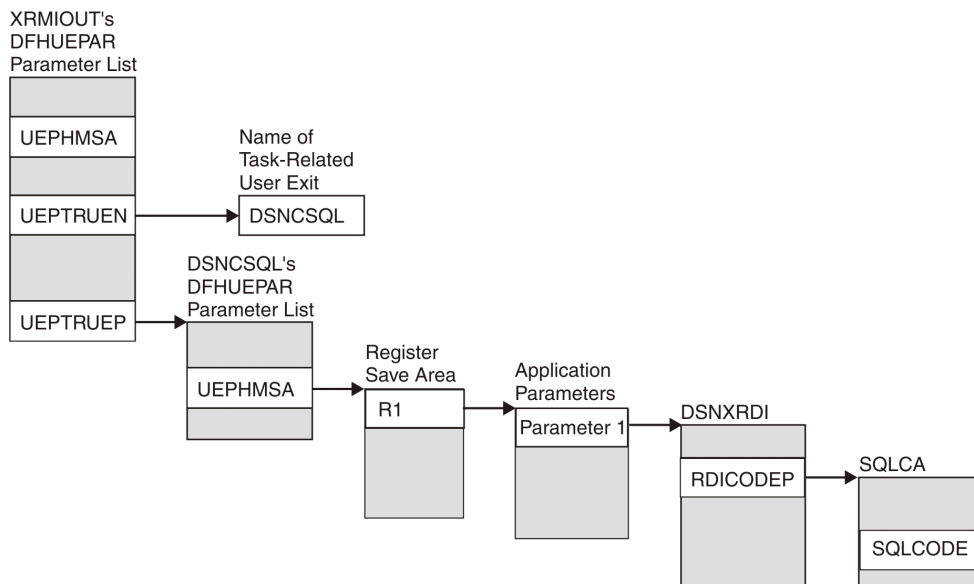
Figure 82. Pointers to resource manager name and SQLCODE
