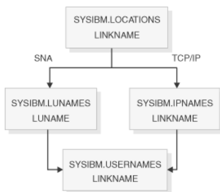
Figure 123. The LINKNAME column of SYSIBM.LOCATIONS determines protocol
