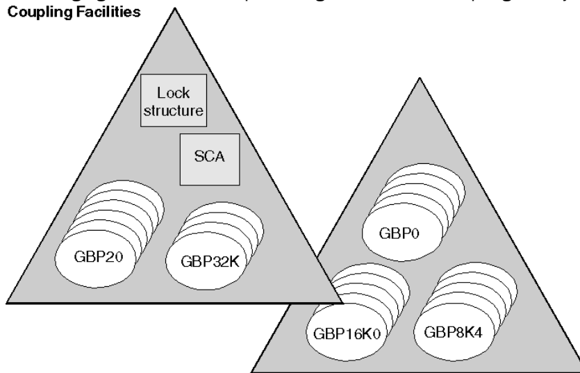
Figure 78. Coupling facility structures that are used by Db2
